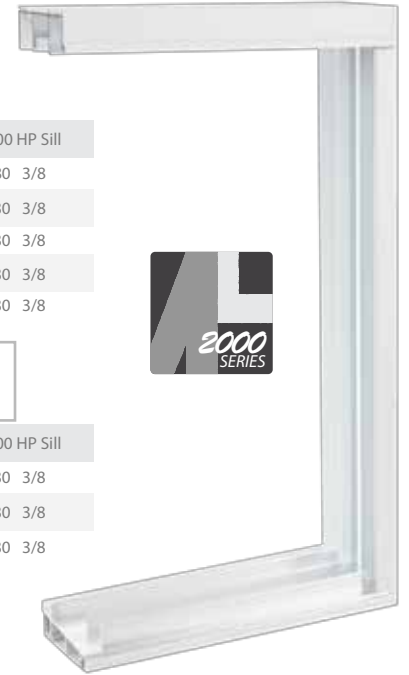
2000 Series optional trailer flange
